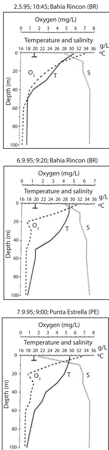
Fig. 2. Profiles of temperature (°C), salinity (UPS) and oxygen concentration ( \text{mgO}_2\cdot\text{L}^{-1} ) at the sampling stations, Golfo Dulce, Costa Rica.
